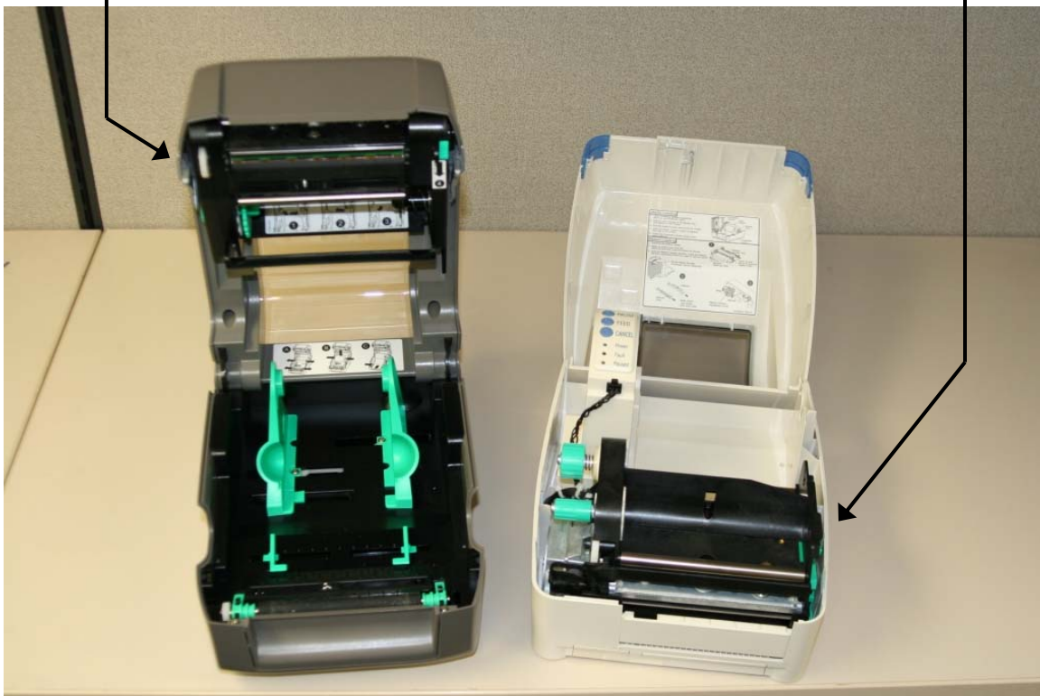
Ribbon Mechanism in Cover
